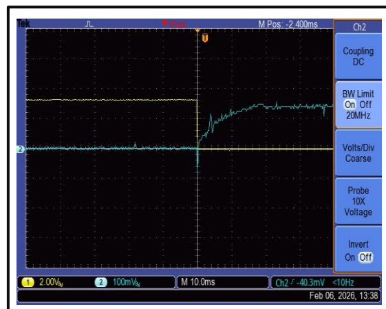
The Drains Open Time is 25 ms @+25°C
