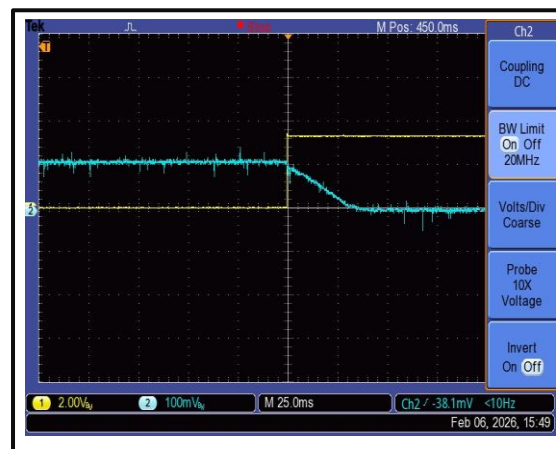
The Drains Closure Time is 35 ms @+25°C
