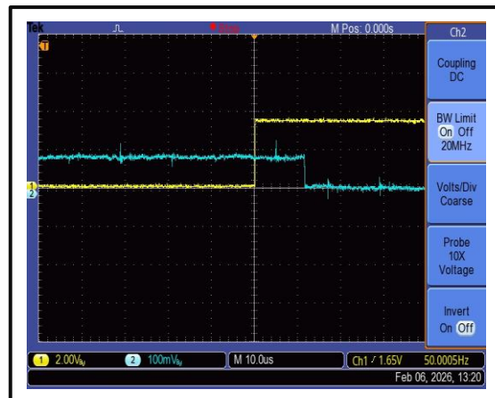
The RF Switch Off Time is 12 us @+25°C
