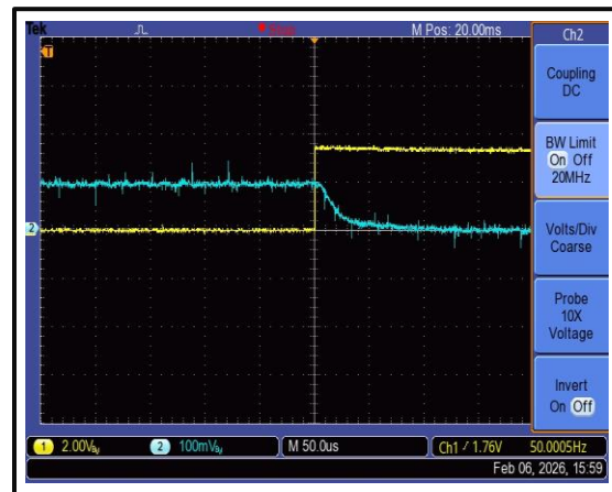
The Gates Closure Time is 150 us @+25°C
