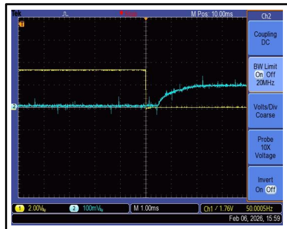
The Gates Open Time is 2500 us @+25°C
