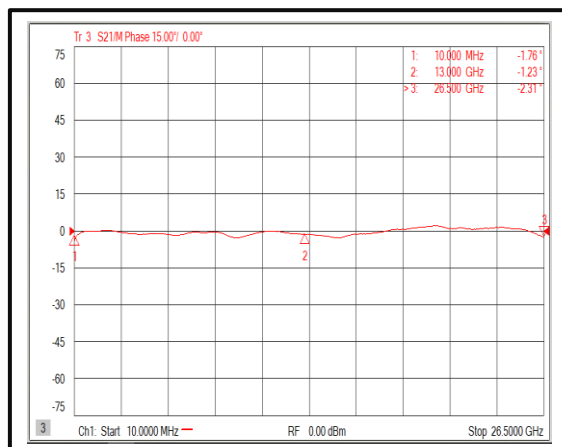
Phase Imbalance
