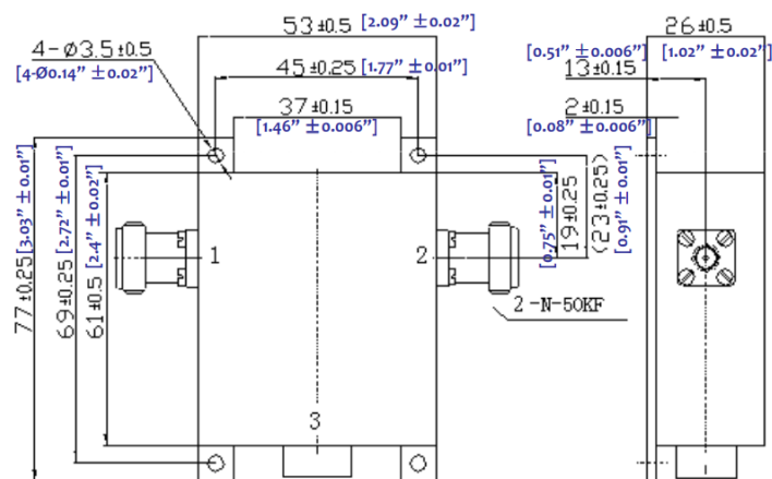
N-Female Version
