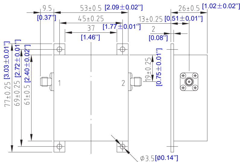
SMA-Female Version
