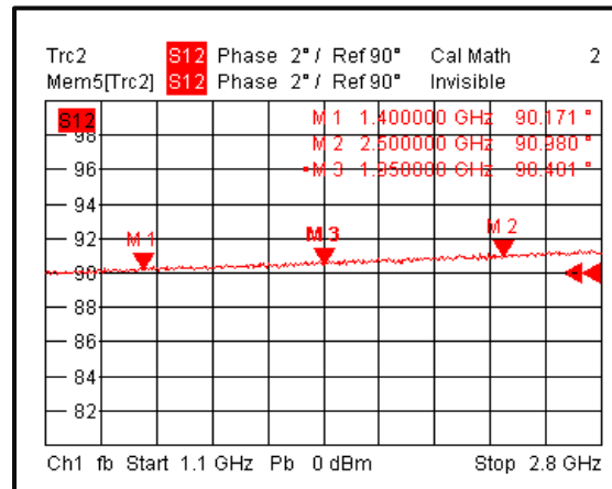
Phase Imbalance
