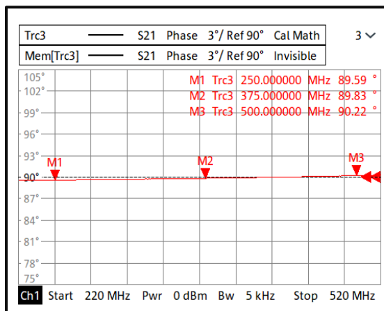
Phase Imbalance
