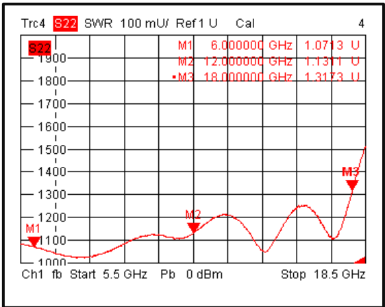
Secondary VSWR 2
