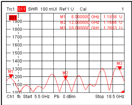
Primary VSWR 2
