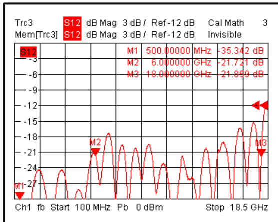
Directivity 2
