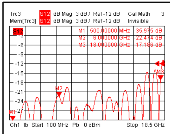
Directivity 1
