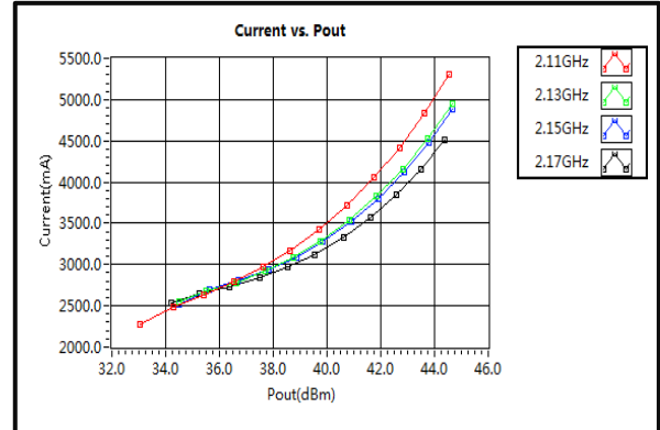
Current vs. Pout (TX)
