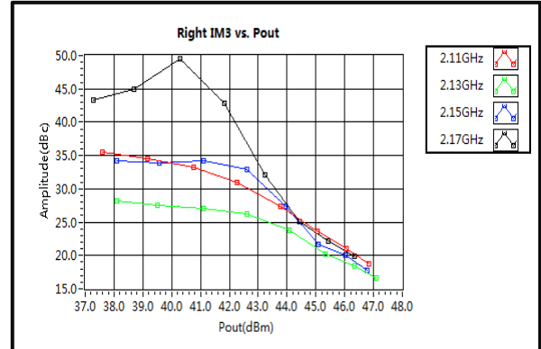
Right IM3 vs. Pout (TX)
