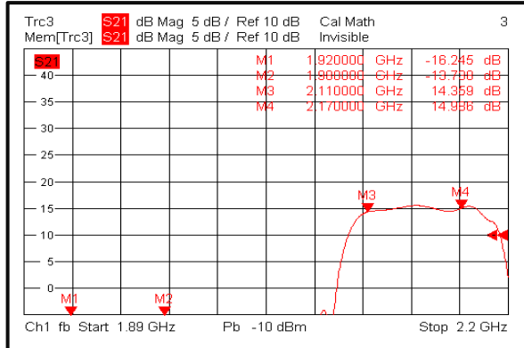
Gain@+25°C (TX)
