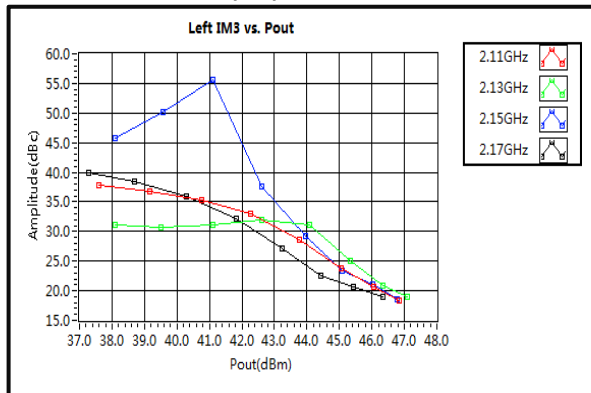
Left IM3 vs. Pout (TX)
