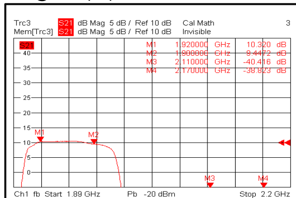
Gain@+25°C (RX)
