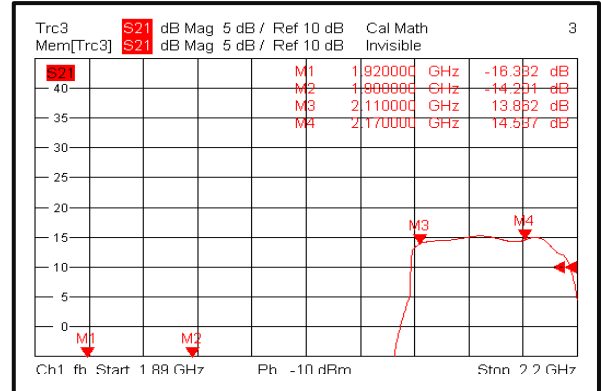
Gain@-10°C (TX)
