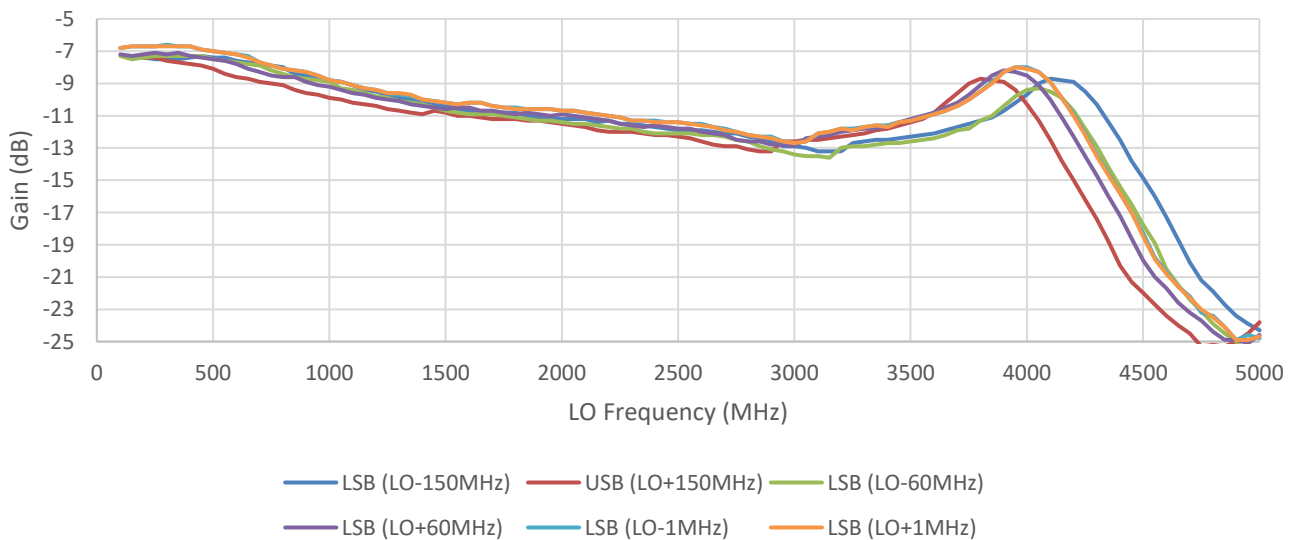
Upconversion Gain with Input Signals 1MHz, 60MHz, 150MHz
