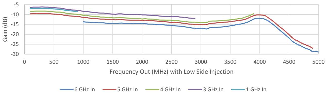
Downconversion Gain with various RF Input Frequencies using Low Side LO Injection ( R_{Fout} = R_{Fin} - LO )
