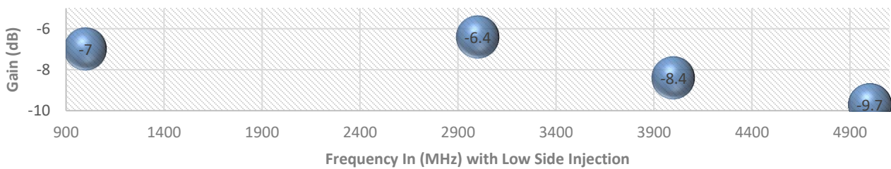
Downconversion Gain to 100MHz RF out
