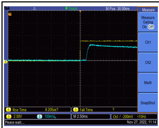
The Gate-Enable Rise Time is 2000 us @+25°C
