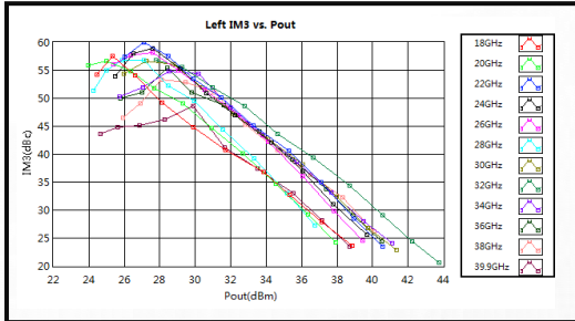
Left IM3 vs. Pout
