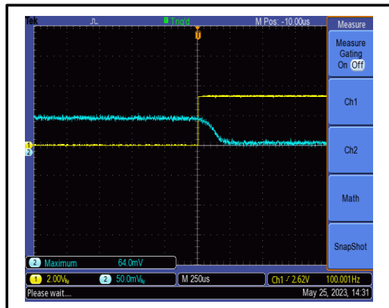
The Gate-Enable Rise Time is 200 us @+25°C
