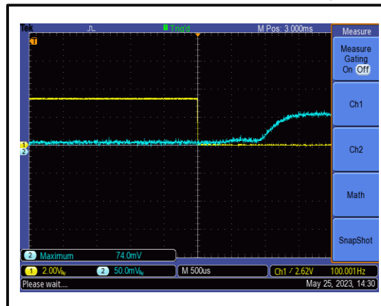
The Gate-Enable Fall Time is 1300 us @+25°C
