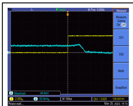
The Drain-Enable Rise Time is 150 us @+25°C
