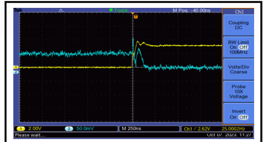
The RF Switch Off Time is 200 ns
