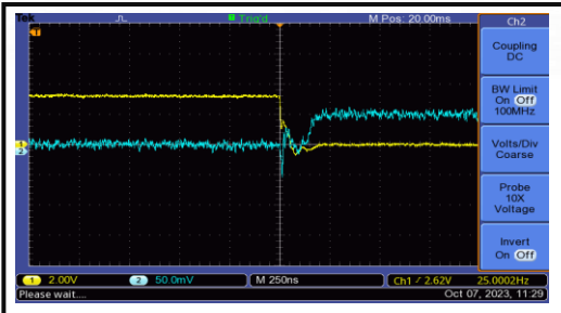
The RF Switch On Time is 200 ns
