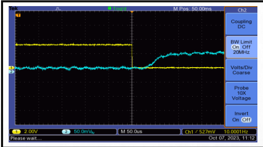
The Gates Open Time is 100 us
