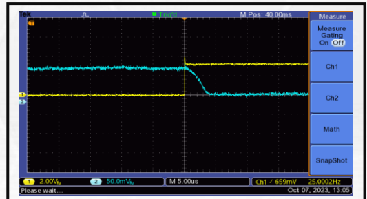
The Drains Closure Time is 5 us
