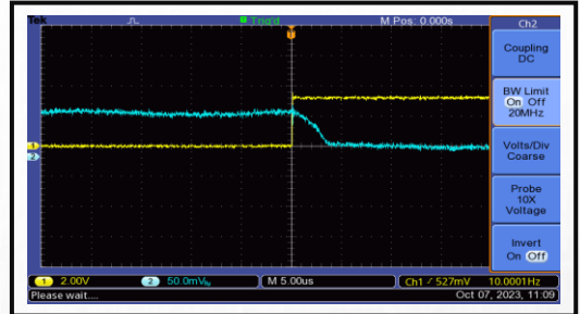
The Gates Closure Time is 5 us
