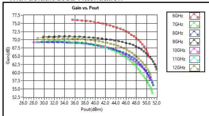
Gain vs Output Power CW With default 10dB Attenuation
