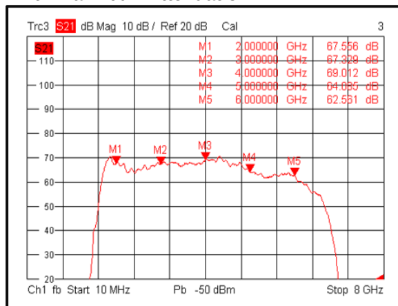
Gain vs. Frequency @+25°C With max 20dB Attenuation
