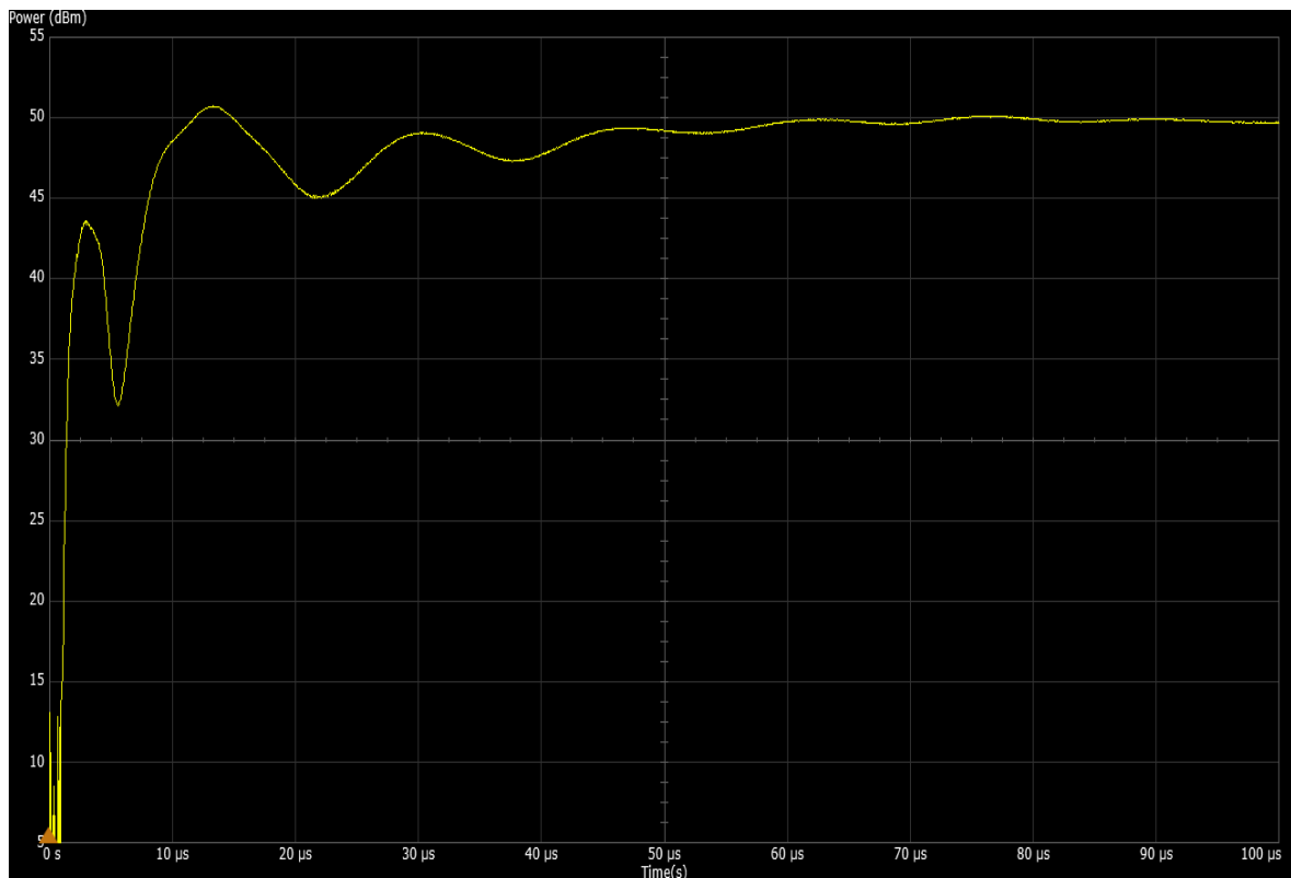
Blanking RF on timing: 50dBm Output Power (10 us/div)
