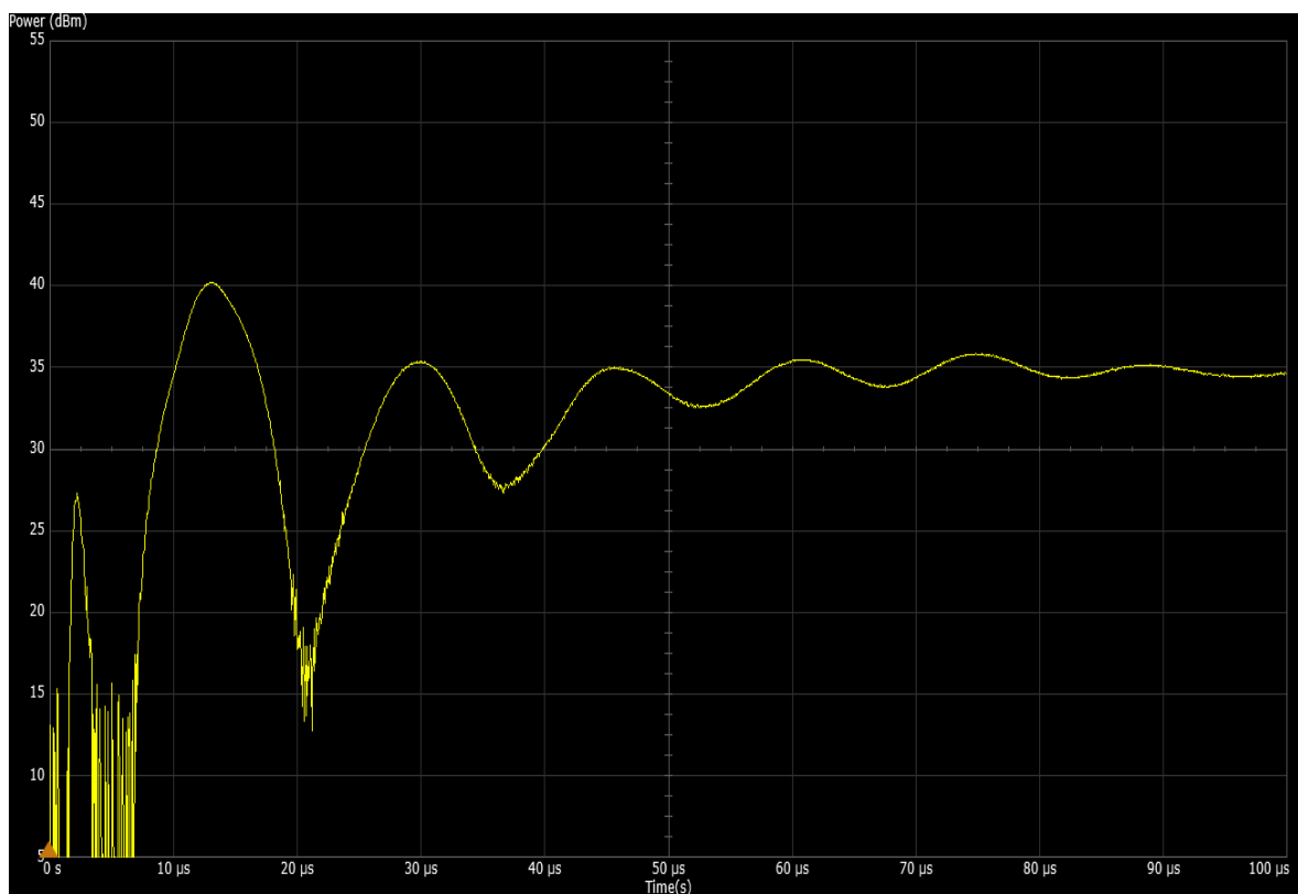
Blanking RF on timing: 40dBm Output Power (10 us/div)
