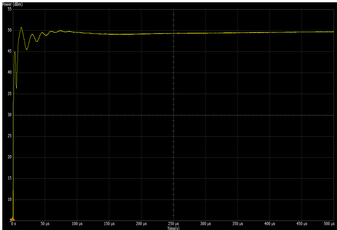
Blanking RF on timing: 50dBm Output Power (50 us/div)
