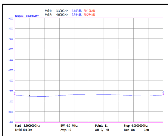
Noise Figure(3.3GHz-4GHz)
