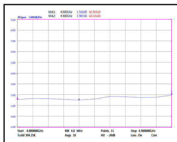
Noise Figure(4GHz-4.9GHz)
