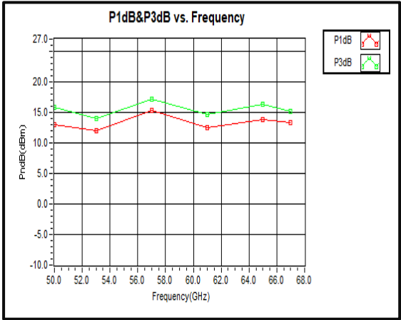
P1dB and P3dB vs. Frequency
