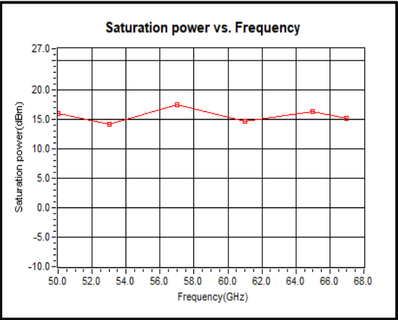
Psat vs. Frequency
