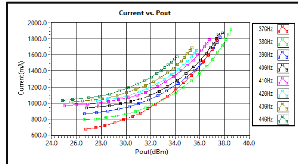
Current vs. Output Power (+24V DC current)
