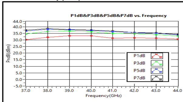
PxdB vs. Freq (CW)
