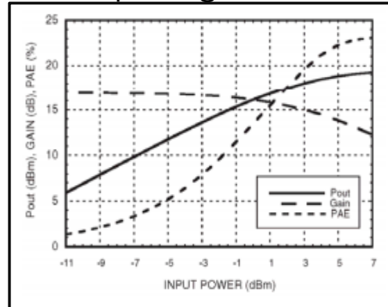
Power Compression @5.5GHz
