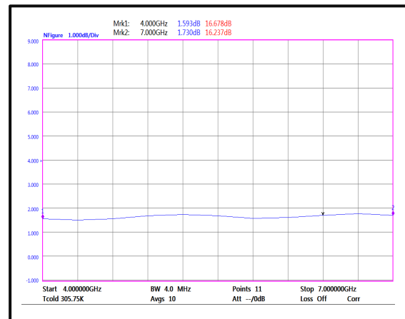
Noise Figure(4-7GHz)
