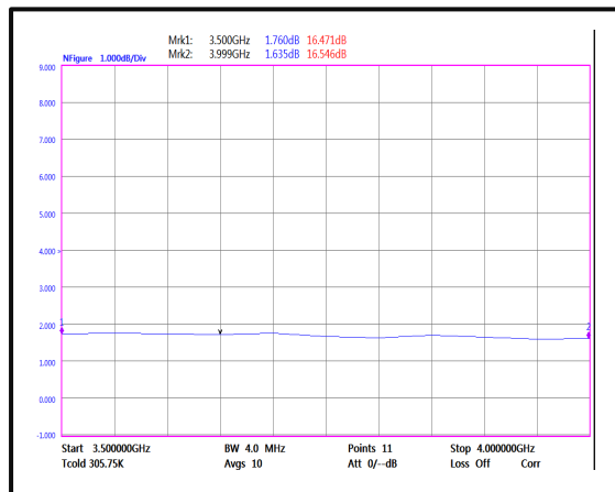
Noise Figure(3.5-4GHz)
