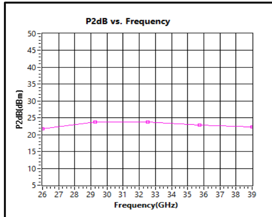
P2dB vs. Frequency
