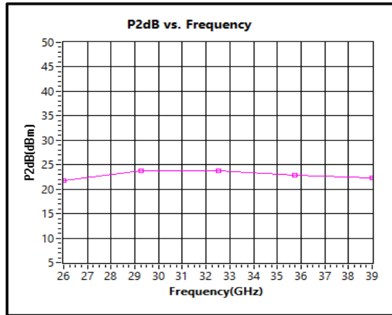
P2dB vs. Frequency
