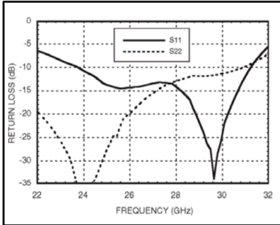
Return Loss
