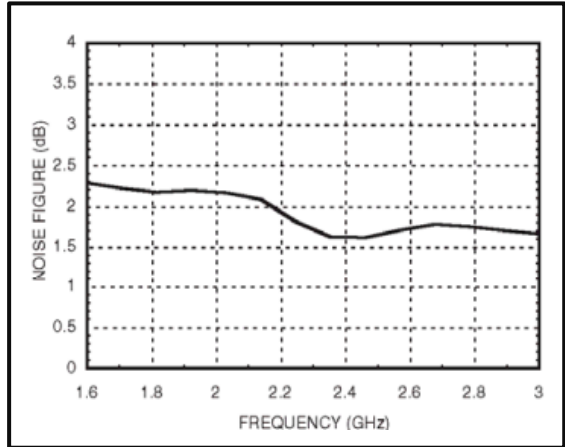
Broadband Noise Figure
