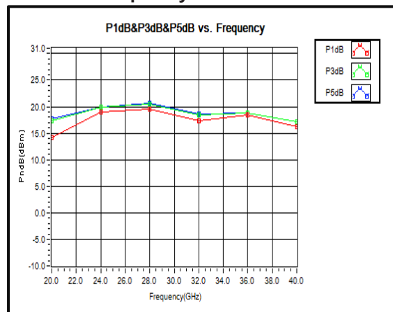
PxdB vs. Frequency
