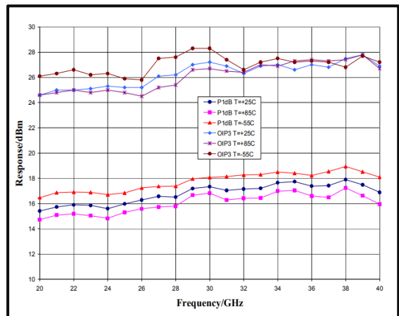
P1dB & Output IP3 vs. Temperature
