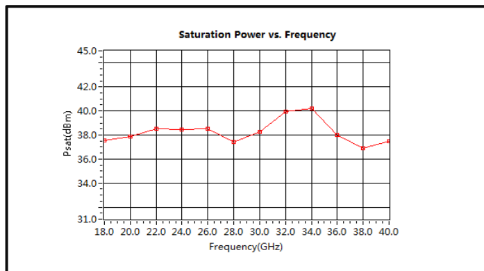
Saturated Power vs. Frequency
