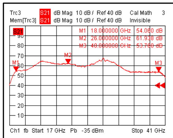
Gain@-30°C
