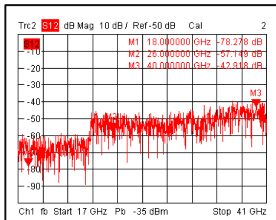
Isolation@-30°C
