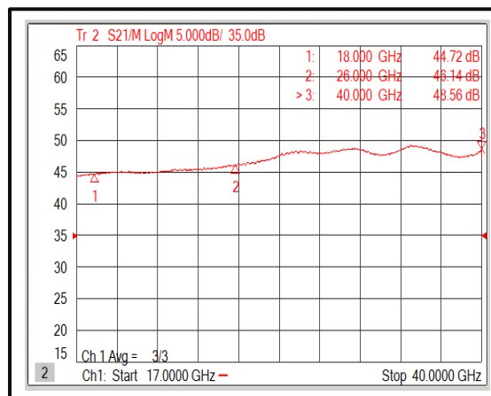
Gain @-30°C
