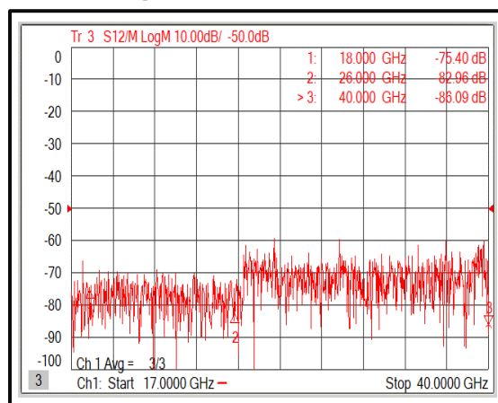
Isolation @-30°C
