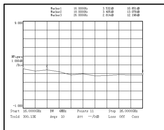
Noise Figure
