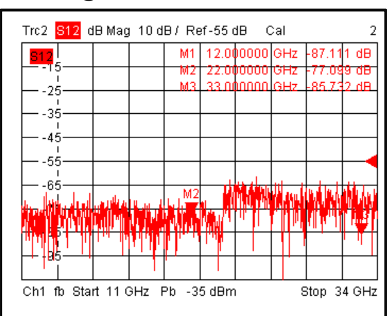
Isolation@-40°C
