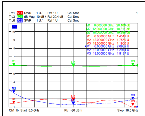
Gain & VSWR
