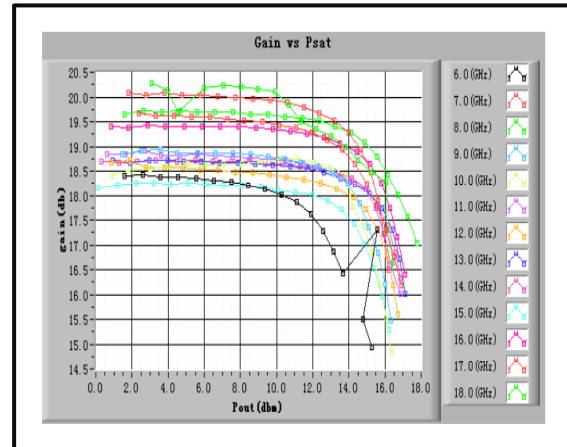
Gain vs. Psat
