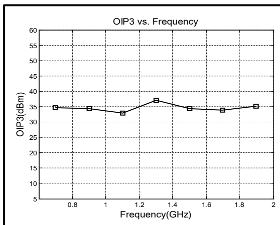
Output Third Order Intercept (IP3)
