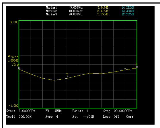
Noise Figure (3-20GHz)
