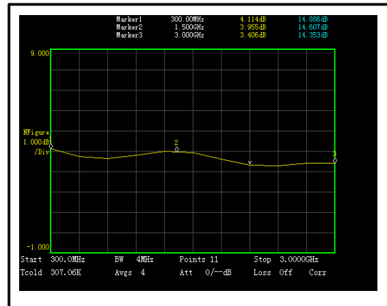
Noise Figure (0.3-3GHz)
