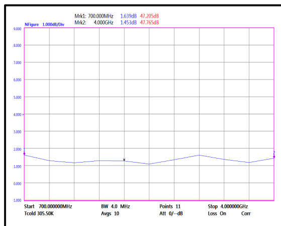
Noise Figure(0.7-4GHz)
