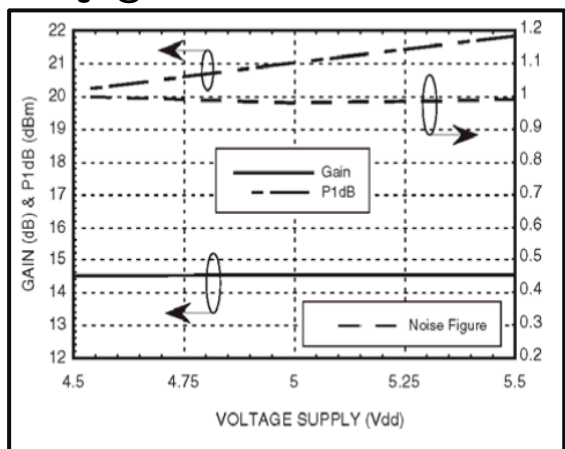
Gain, Noise Figure & Power vs. Supply Voltage @850MHz
