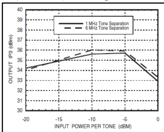
Output IP3 vs. Input Power @950MHz
