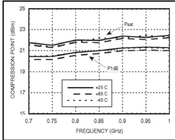
P1dB & Psat vs. Temperature
