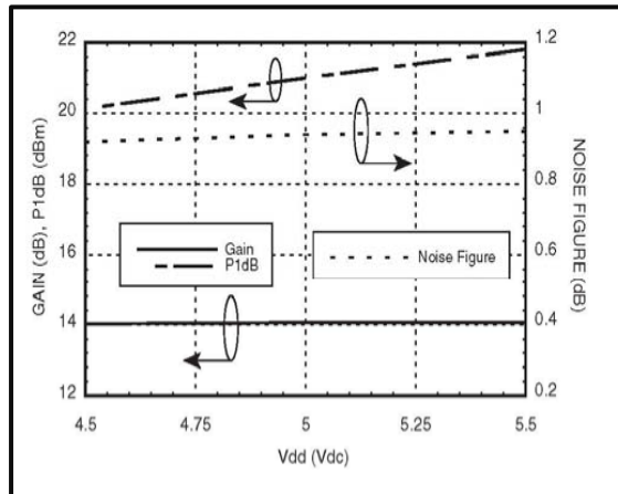
GAIN, Noise Figure Power vs. Supply Voltage @850 MHz
