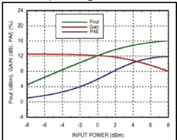
Power Compression @24GHz
