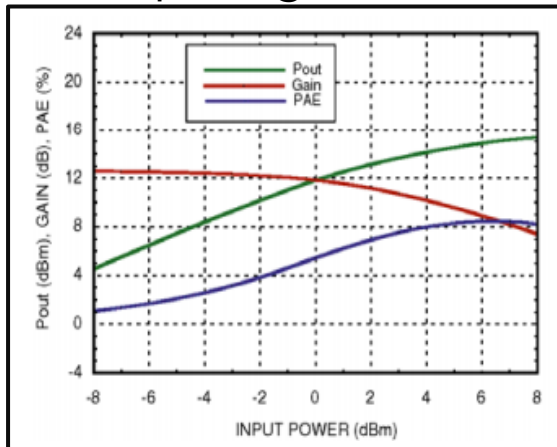
Power Compression @17GHz
