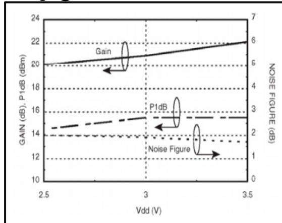
Gain, Power & Noise Figure vs. Supply Voltage @12GHz
