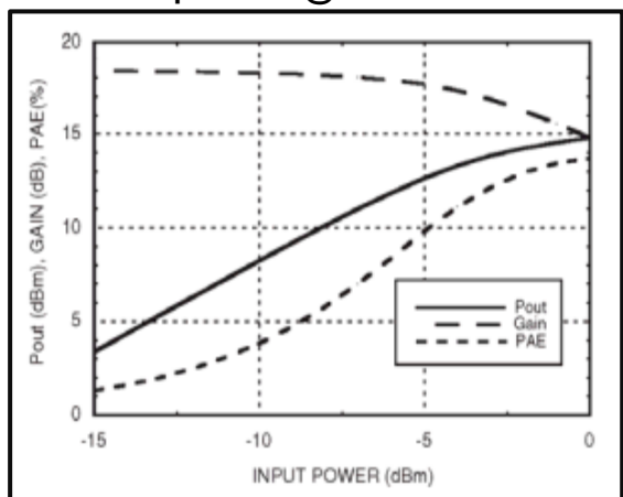
Power Compression @8GHz
