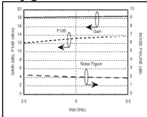
Gain, Power & Noise Figure vs. Supply Voltage @8GHz
