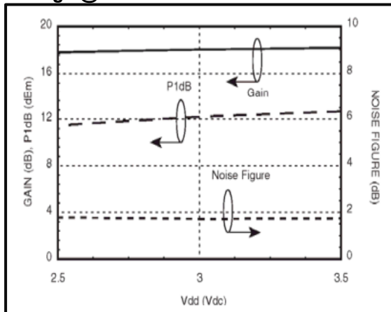
Gain, Noise Figure & Power vs. Supply Voltage @8GHz
