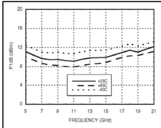
P1dB vs.Temperature
