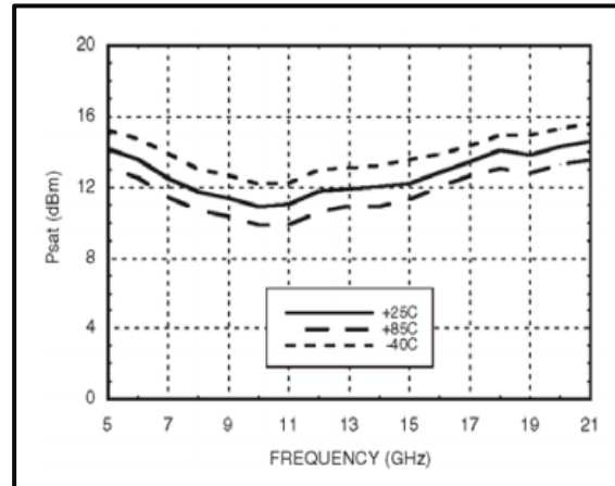
Psat vs.Temperature
