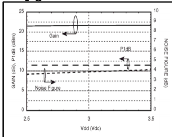
Gain, Noise Figure & Power vs Supply Voltage @12GHz
