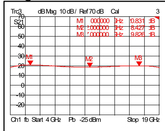
Gain @-40°C
