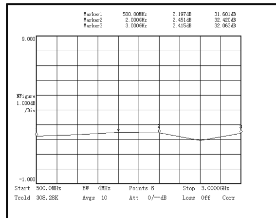
Noise Figure(500MHz-3GHz)
