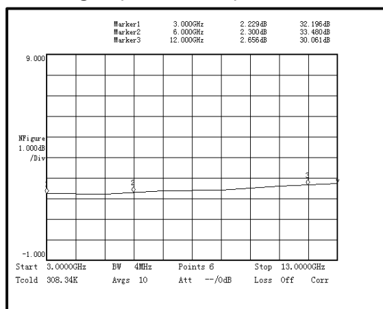
Noise Figure(3GHz-13GHz)
