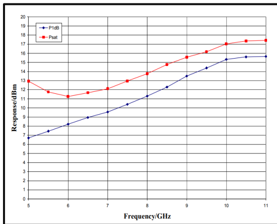
Output Power
