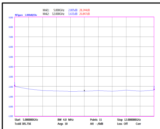
Noise Figure
