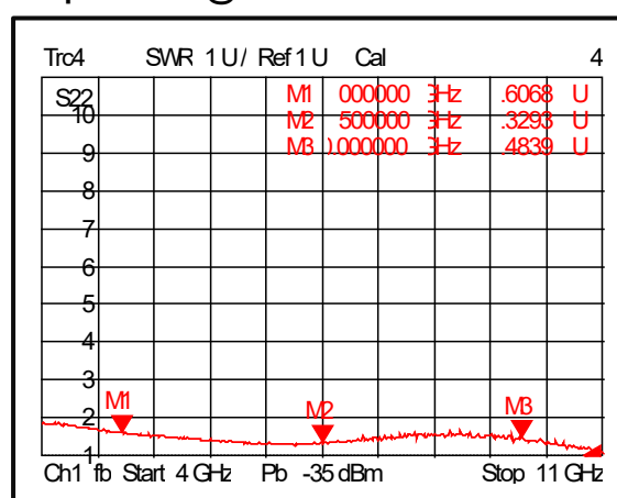
Output VSWR@+85°C
