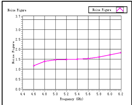
Noise Figure
