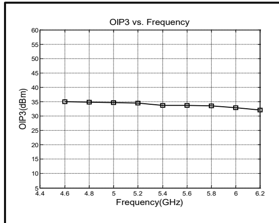
Output Third Order Intercept (IP3)
