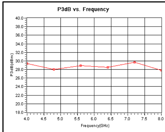
P3dB vs. Frequency
