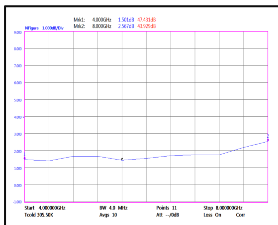
Noise Figure (4GHz-8GHz)
