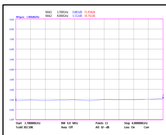
Noise Figure(3.7-4GHz)
