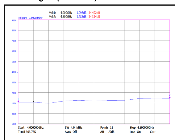
Noise Figure(4-4.5GHz)
