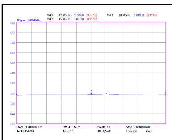
Noise Figure
